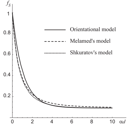
Fig. 11. Diffuse nonabsorbance f_S given by our model (solid curve), Melamed's model (dashed curve), and the model of Shkuratov et al. (dotted curve) as functions of the diametrical absorbance.
