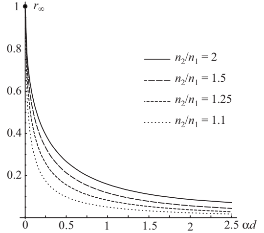
Fig. 7. Infinite particle medium reflectance as a function of diametrical absorbance for various relative refractive indices with a shadowing ratio a=0.5 .
