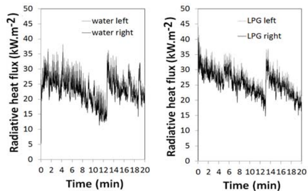
Figure 3: Heat flux impacting the tank with water (left) or propane (right)
