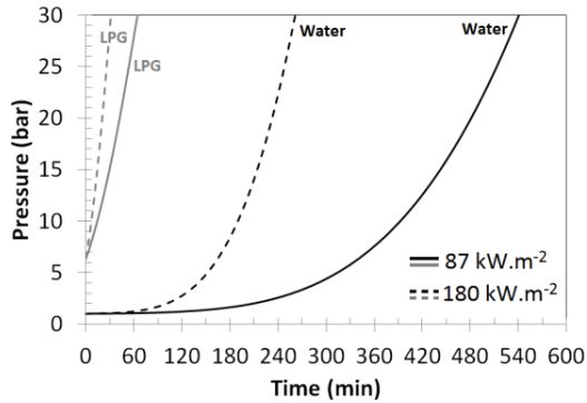
Figure 8: Pressure increase with temperature
